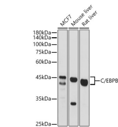
Western blot analysis of extracts of various cell lines, using C/EBPB antibody (STJ111016) at 1:500 dilution. Secondary antibody: HRP Goat Anti-rabbit IgG (H+L) at 1:10000 dilution. Lysates/proteins: 25µg per lane. Blocking buffer: 3% nonfat dry milk in TBST. Detection: ECL Basic Kit. Exposure time: 30s.
