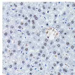
Immunohistochemistry of paraffin-embedded rat liver using C/EBPB rabbit polyclonal antibody (STJ111016) at dilution of 1:100 (40x lens). Perform high pressure antigen retrieval with 10 mM citrate buffer pH 6, 0 before commencing with immunohistochemistry staining protocol.
