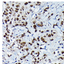
Immunohistochemistry of paraffin-embedded human breast cancer using C/EBPB rabbit polyclonal antibody (STJ111016) at dilution of 1:100 (40x lens). Perform high pressure antigen retrieval with 10 mM citrate buffer pH 6, 0 before commencing with immunohistochemistry staining protocol.
