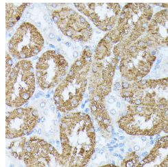
Immunohistochemistry of paraffin-embedded rat kidney using PLS1 antibody (STJ117498) at dilution of 1:100 (40x lens).
