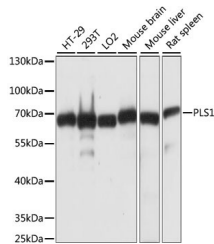
Western blot analysis of extracts of various cell lines, using PLS1 antibody (STJ117498) at 1:1000 dilution. Secondary antibody: HRP Coated Anti-rabbit IgG (H+L) at 1:10000 dilution. Lysates/proteins: 25ug per lane. Blocking buffer: 3% nonfat dry milk in TBST. Detection: ECL Basic Kit. Exposure time: 3s.
