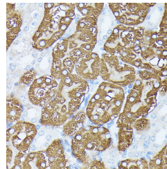
Immunohistochemistry of paraffin-embedded mouse kidney using PLS1 antibody (STJ117498) at dilution of 1:100 (40x lens).
