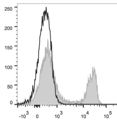
Rat splenocytes were stained with Anti-CD4 (domain 1) antibody (STJA0000606) (filled gray histogram). Unstained splenocytes (empty black histogram) were used as control.
