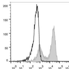
C57BL/6 murine splenocytes were stained with Anti-TCR \beta antibody (STJA0000778) [Used at 0.05 \mu g/ 10^6 cells dilution] (filled gray histogram). Unstained splenocytes (empty black histogram) were used as control.
