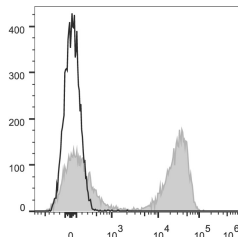
C57BL/6 murine splenocytes were stained with Anti-TCR \beta antibody (STJA0000783) [Used at 0.2 \mu g/ 10^6 cells dilution] (filled gray histogram). Unstained splenocytes (empty black histogram) were used as control.
